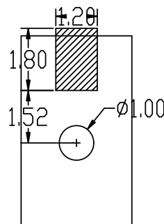
1PIN P.C.B. LAYOUT (TOP VIEW)
